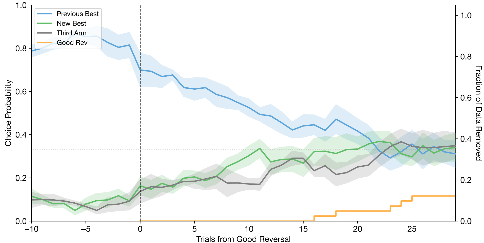
Good Reversal-Aligned Choices (mean \pm se across subjects | n=8 subjects, n=41 reversals)
